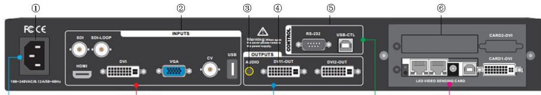
Figure 1-Video processor rear panel
