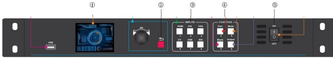
Figure 3-Front Panel
